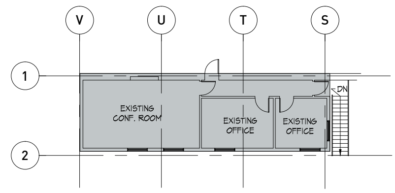
MEZZANINE- OFFICE AREA FLOOR PLAN ±750 SF. NTS
