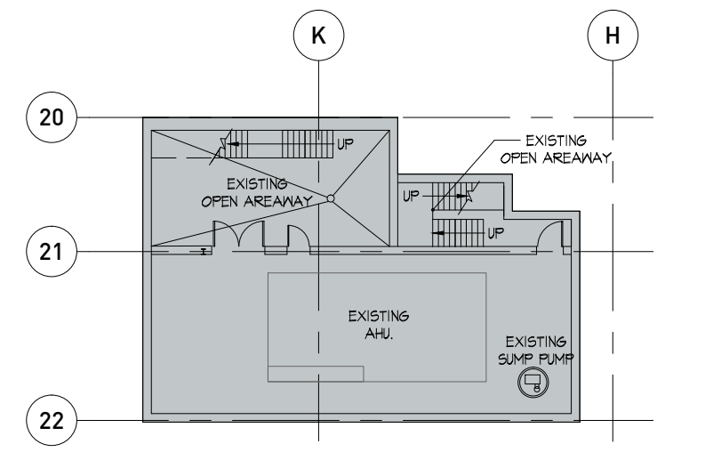
BASEMENT- MECH ROOM FLOOR PLAN ± 1,507 SF. NTS
